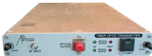
Front view: Optical transmitter
